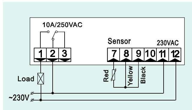
Circuit Diagram
